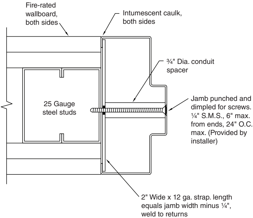
Figure 35 – Countersink mount
