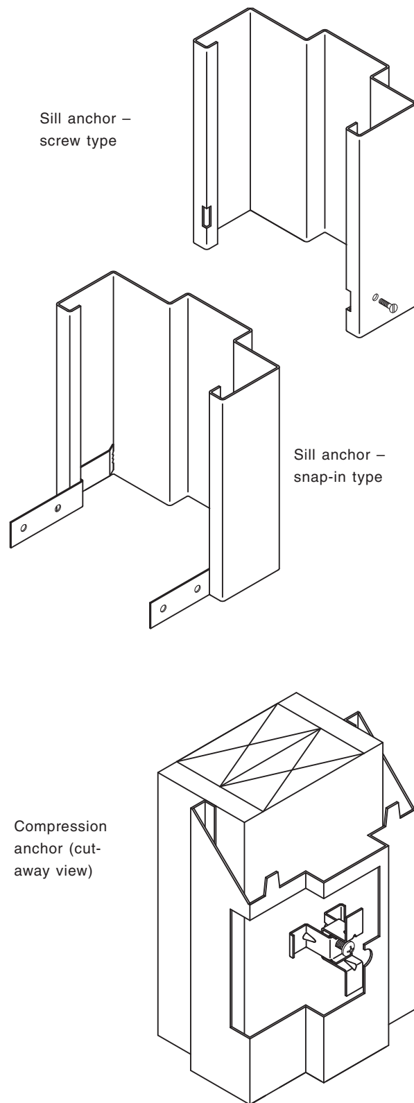
Figure 33 – Fasten base anchors to wall stud
